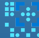
Vector Index
